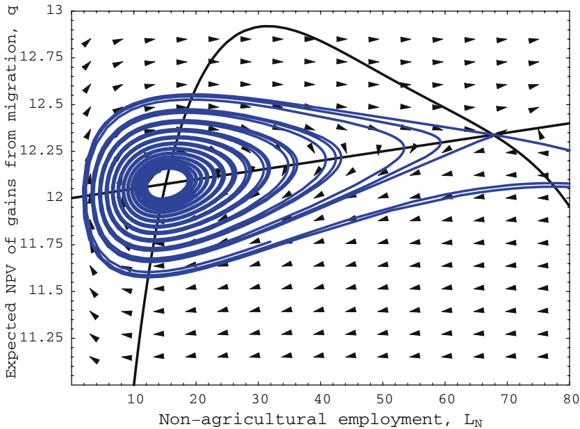
Fig. 6 Expectations and equilibrium stability Notes. The figure depicts the migration dynamics for the system defined by the system of differential Equations (22) and (21). The figure illustrates that under our fully specified migration process both of the interior equilibria are locally stable and thus observable under occasional perturbation. However, our migration model also gives rise to local indeterminacy, generating multiple perfect foresight paths for any given initial labor allocation
