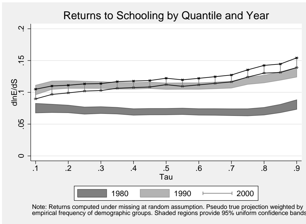
Figure 3: Confidence Intervals Under Missing at Random Assumption
