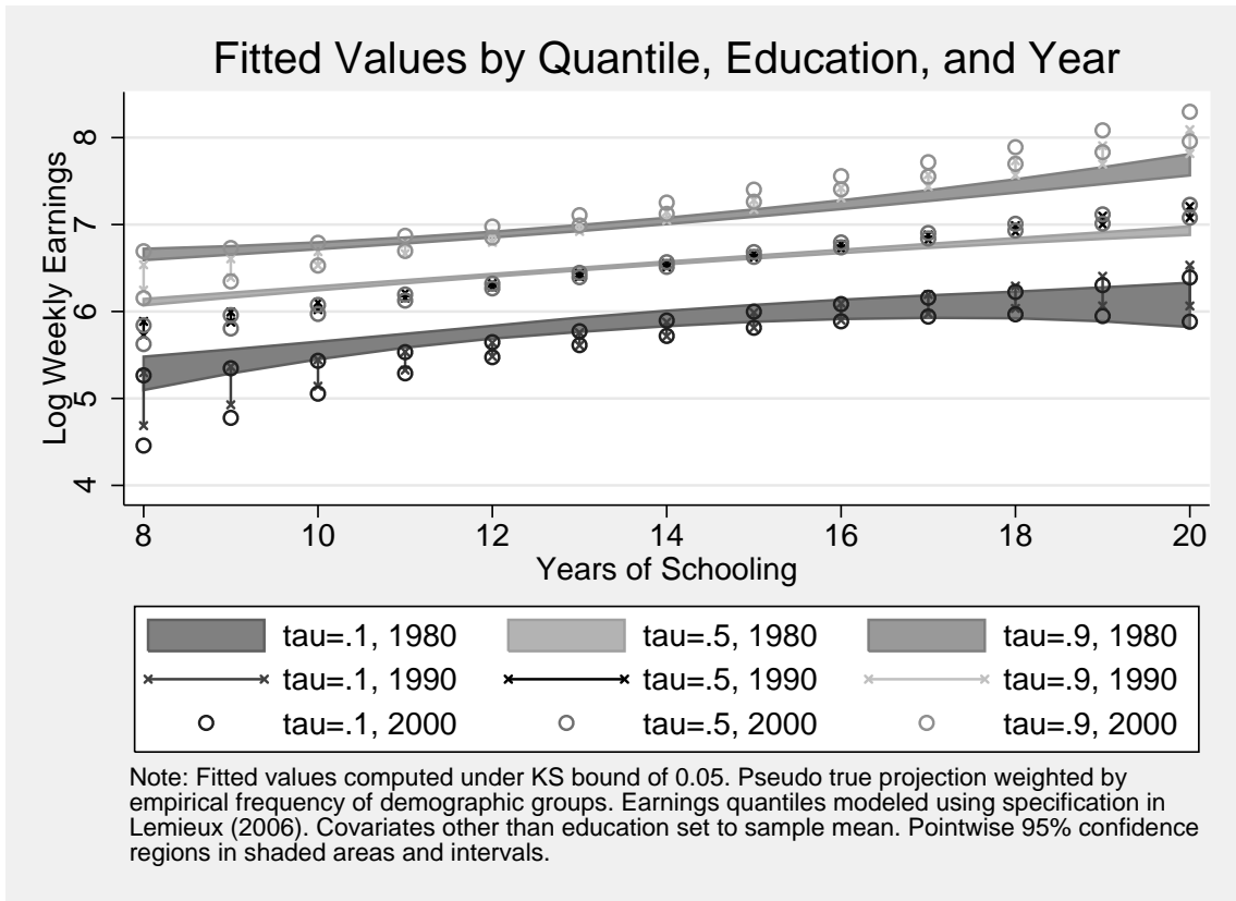
Figure 8: Confidence Intervals for Fitted Values Under \mathcal{S}(F) \leq 0.05
